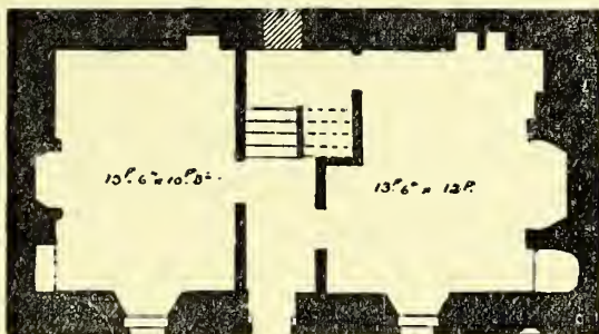
Ground Plan
